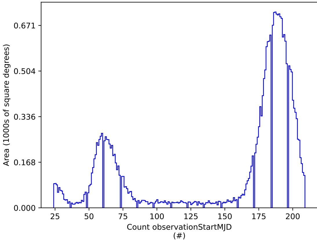
baseline_v3.0_10yrs i: Count observationStartMJD
