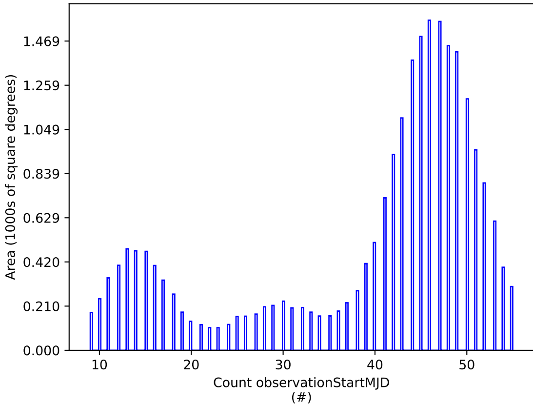
baseline_v3.0_10yrs u: Count observationStartMJD
