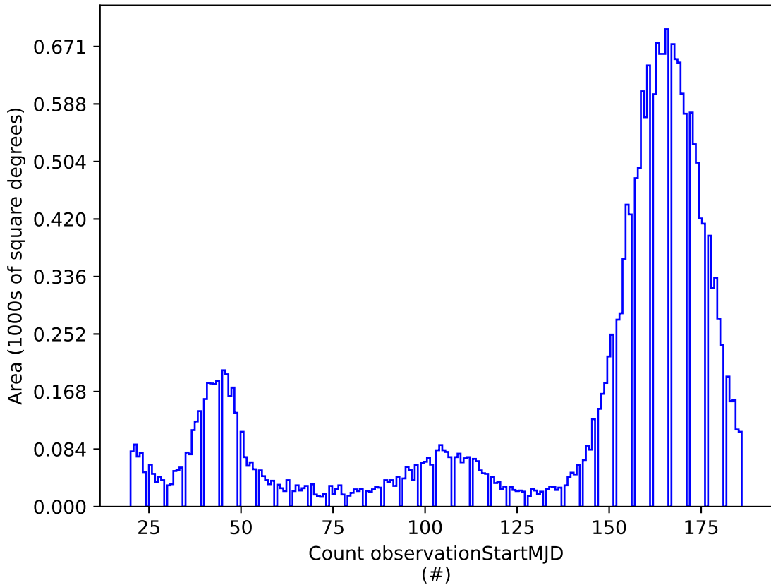
baseline_v3.0_10yrs y: Count observationStartMJD
