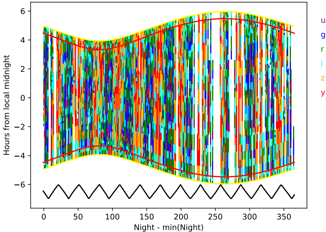
baseline_v3.0_10yrs year 6-7: Hourglass
