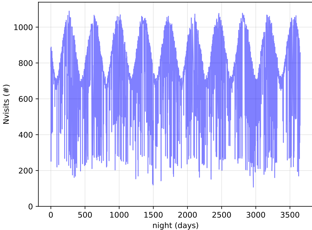
baseline_v3.0_10yrs All visits: Nvisits
