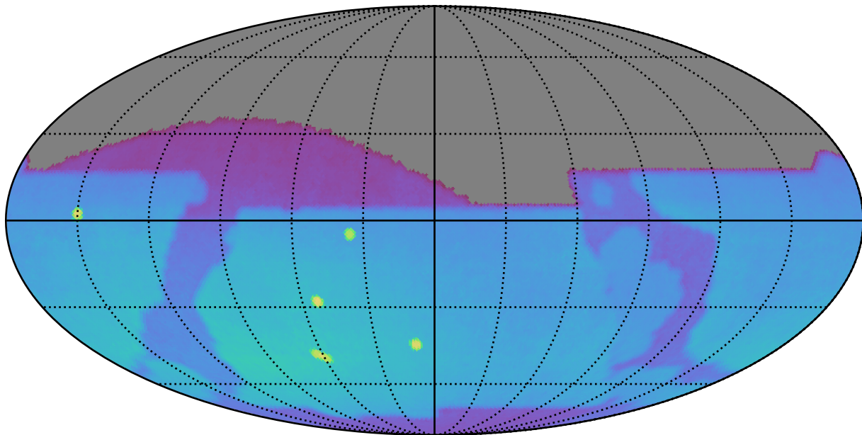
baseline_v3.0_10yrs : Brown Dwarf, L4
