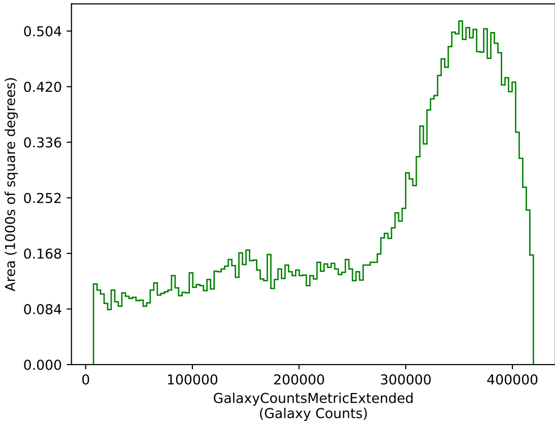
baseline_v3.0_10yrs g: GalaxyCountsMetricExtended
