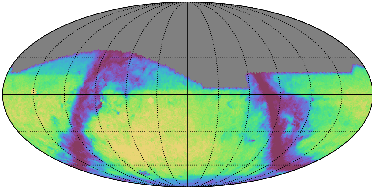
baseline_v3.0_10yrs g: GalaxyCountsMetricExtended
