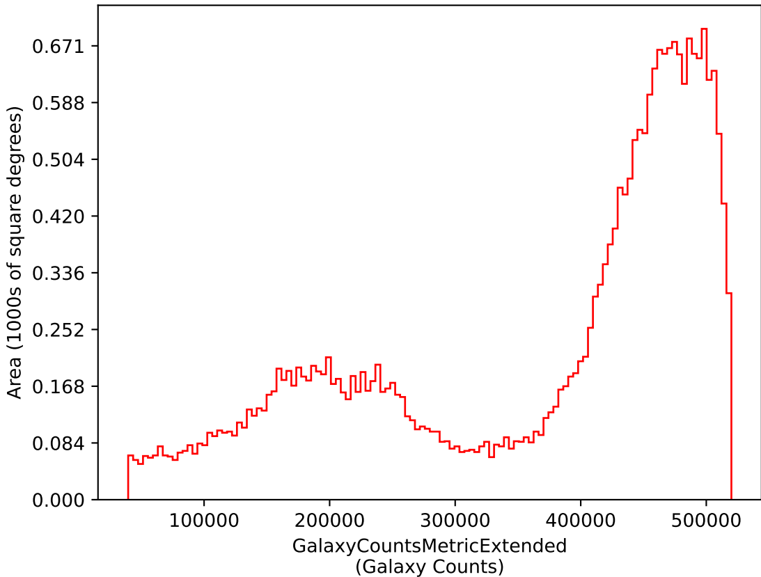
baseline_v3.0_10yrs i: GalaxyCountsMetricExtended
