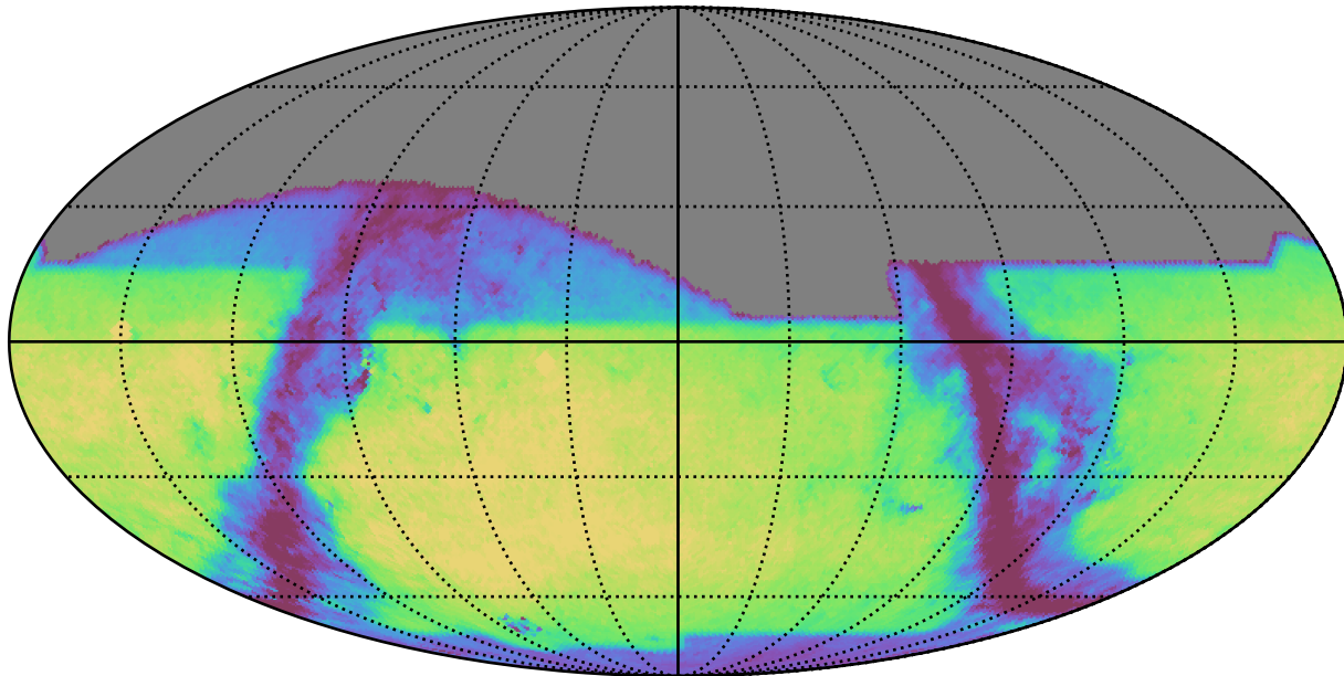
baseline_v3.0_10yrs i: GalaxyCountsMetricExtended
