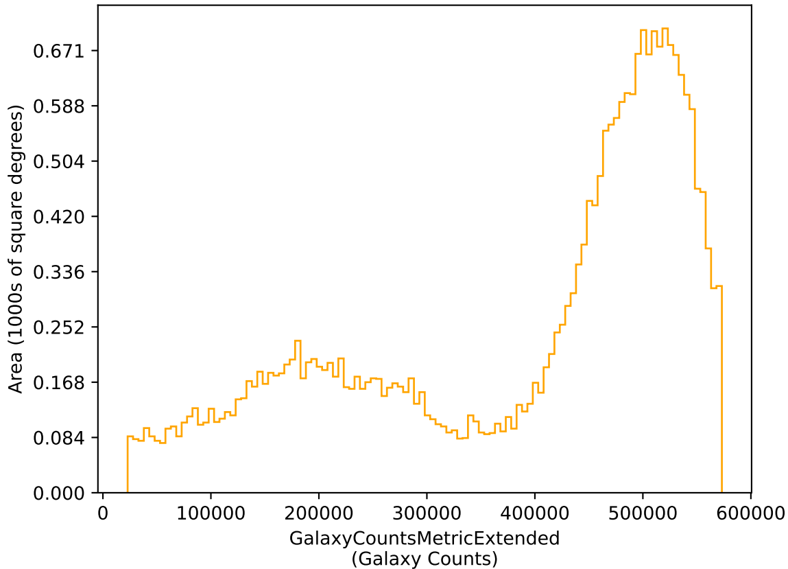
baseline_v3.0_10yrs r: GalaxyCountsMetricExtended
