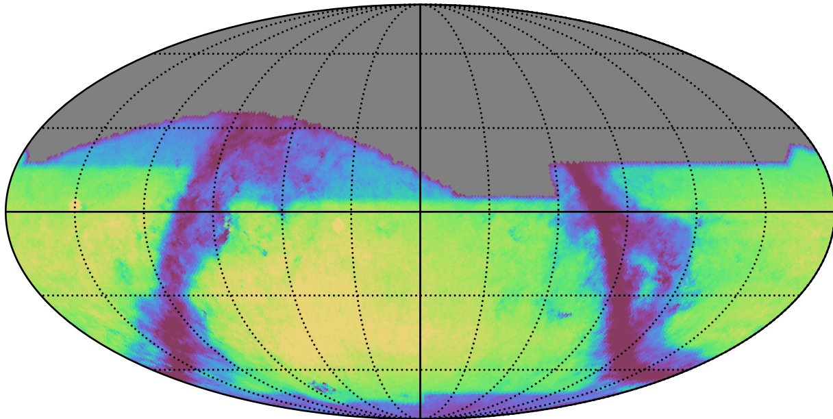
baseline_v3.0_10yrs r: GalaxyCountsMetricExtended
