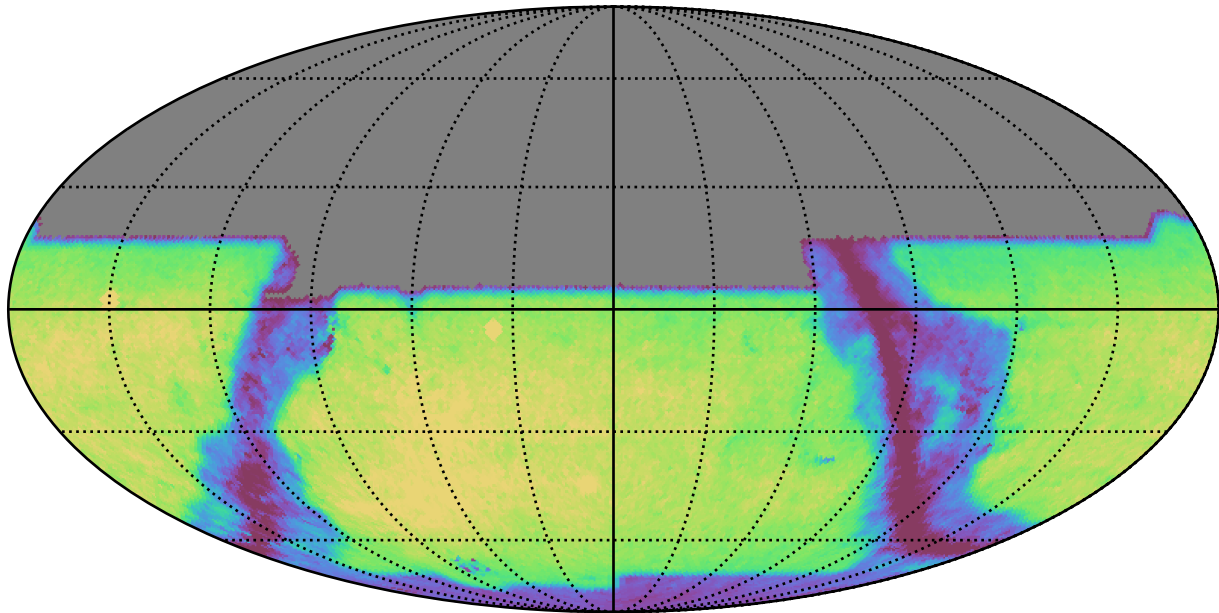
baseline_v3.0_10yrs y: GalaxyCountsMetricExtended
