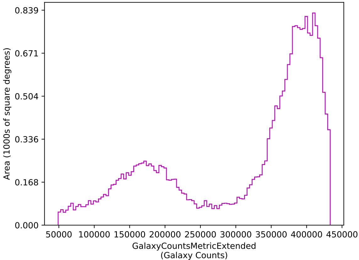
baseline_v3.0_10yrs z: GalaxyCountsMetricExtended
