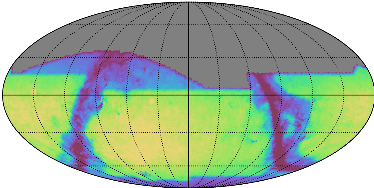
baseline_v3.0_10yrs z: GalaxyCountsMetricExtended
