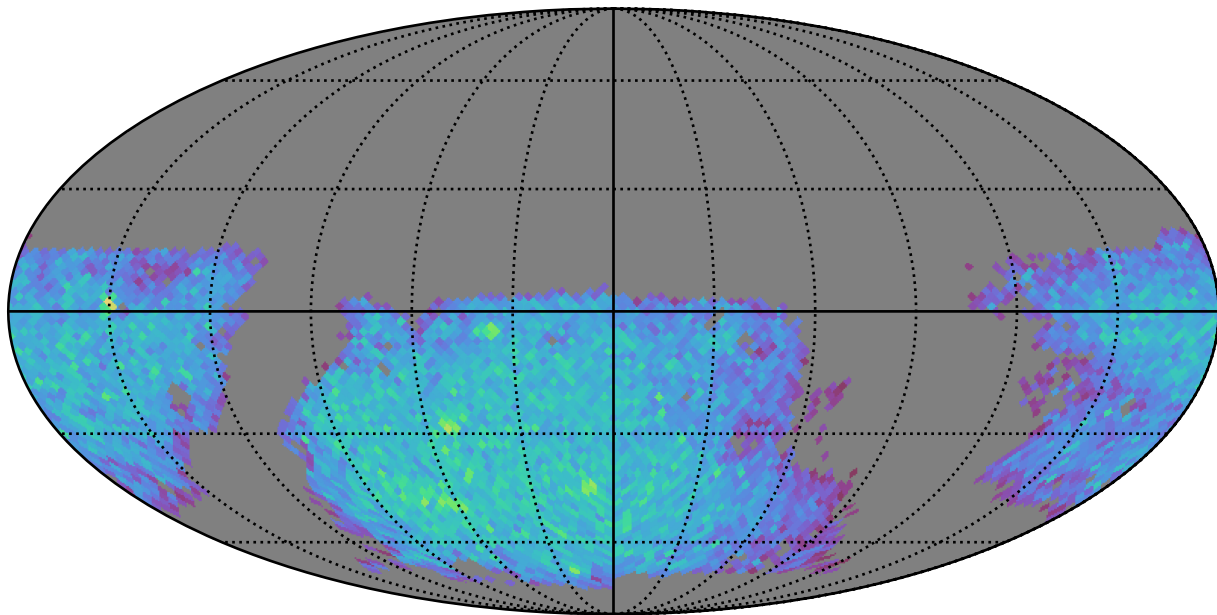
baseline_v3.0_10yrs gi: LVDwarfs
