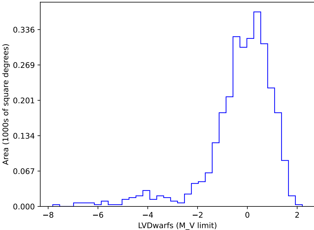
baseline_v3.0_10yrs gi SCP: LVDwarfs
