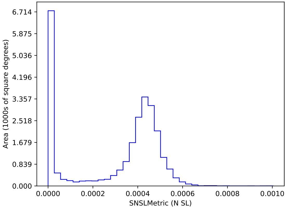
baseline_v3.0_10yrs : SNSLMetric
