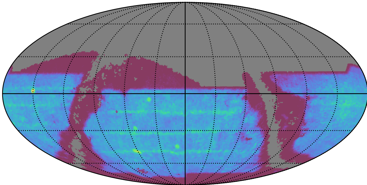
baseline_v3.0_10yrs : SNSLMetric
