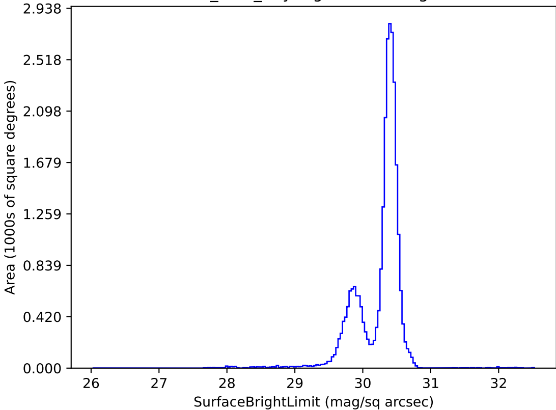
baseline_v3.0_10yrs g: SurfaceBrightLimit
