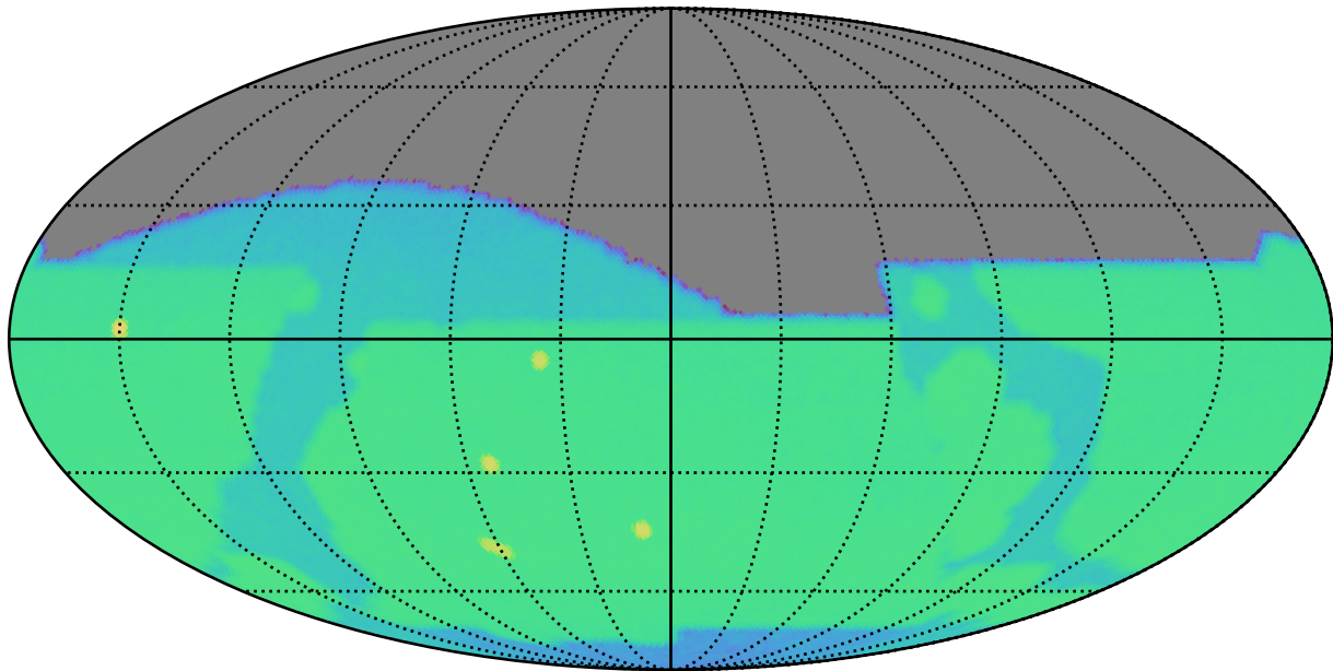
baseline_v3.0_10yrs r: SurfaceBrightLimit
