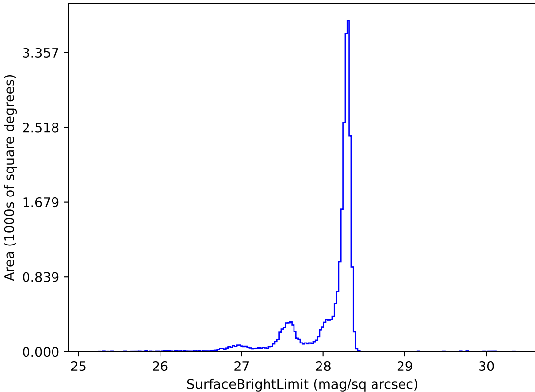
baseline_v3.0_10yrs y: SurfaceBrightLimit
