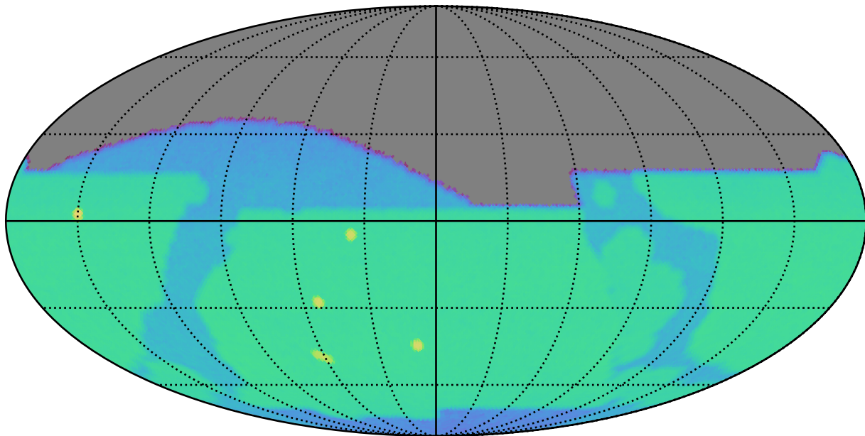
baseline_v3.0_10yrs z: SurfaceBrightLimit
