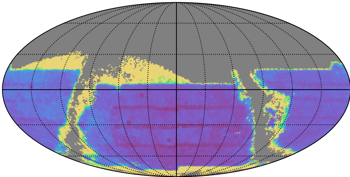
baseline_v3.0_10yrs : TDC_accuracy
