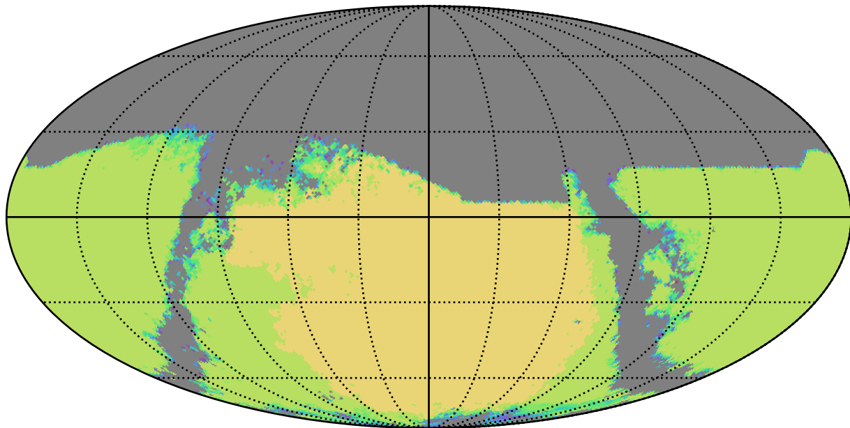
baseline_v3.0_10yrs : TDC_campaign
