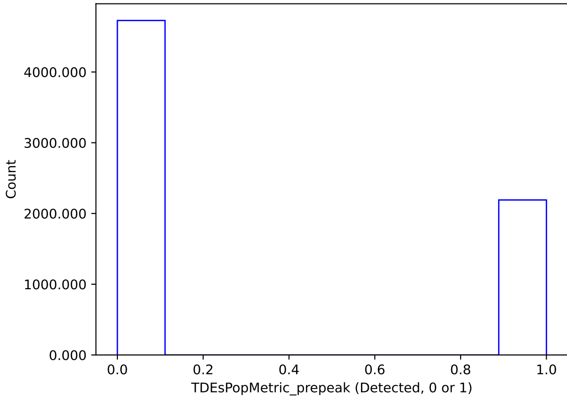
baseline_v3.0_10yrs : TDEsPopMetric_prepeak
