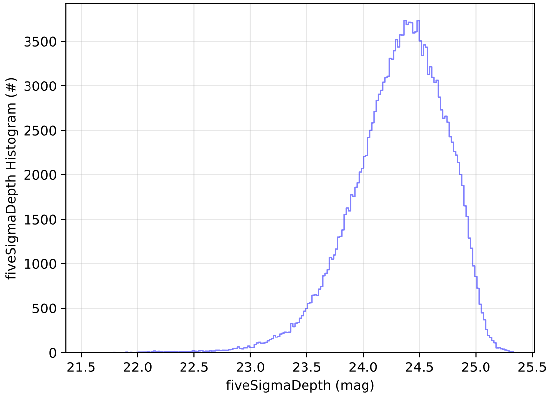
baseline_v3.0_10yrs g: fiveSigmaDepth Histogram
