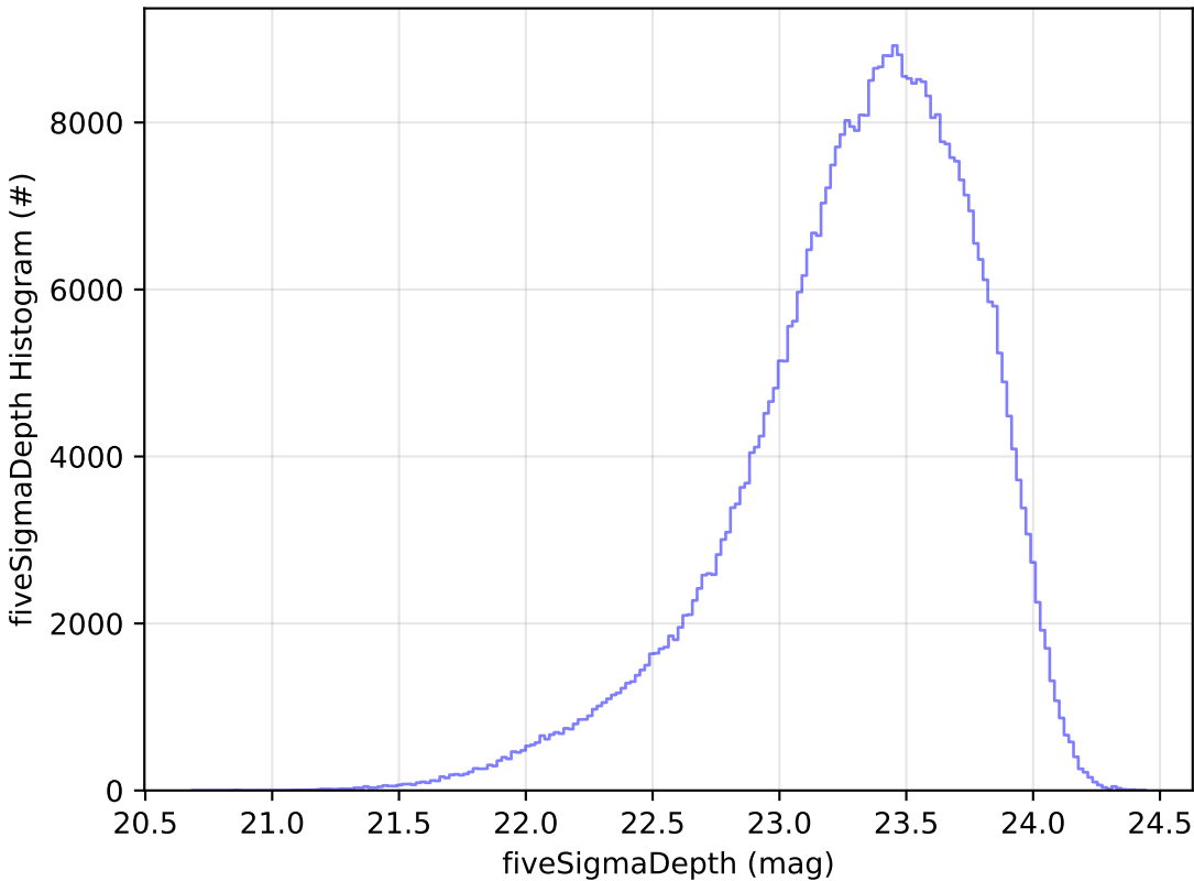
baseline_v3.0_10yrs i: fiveSigmaDepth Histogram
