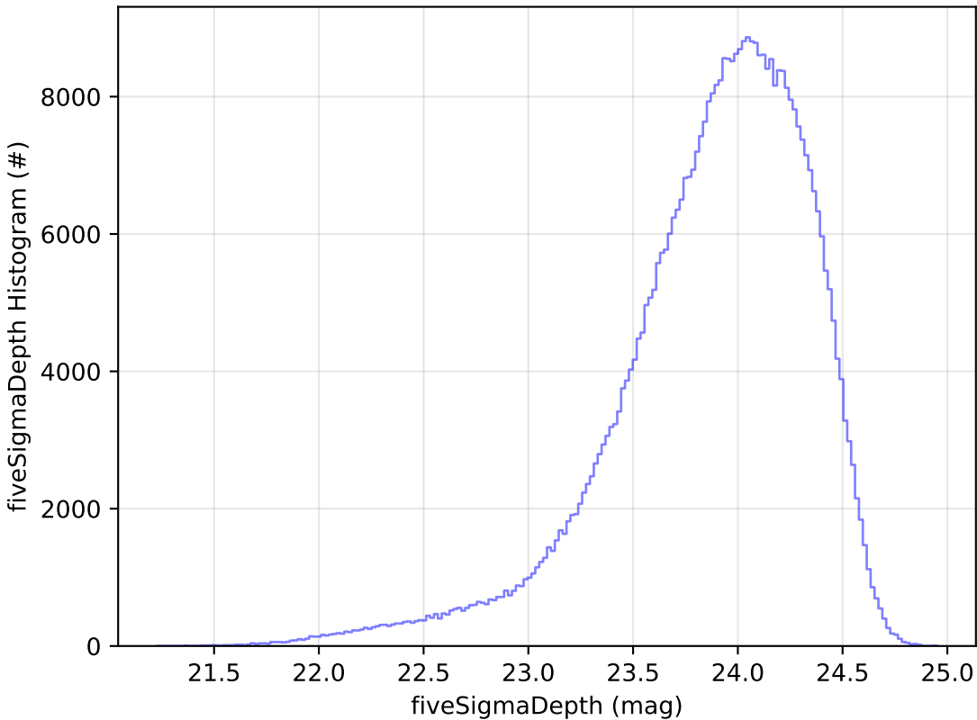
baseline_v3.0_10yrs r: fiveSigmaDepth Histogram
