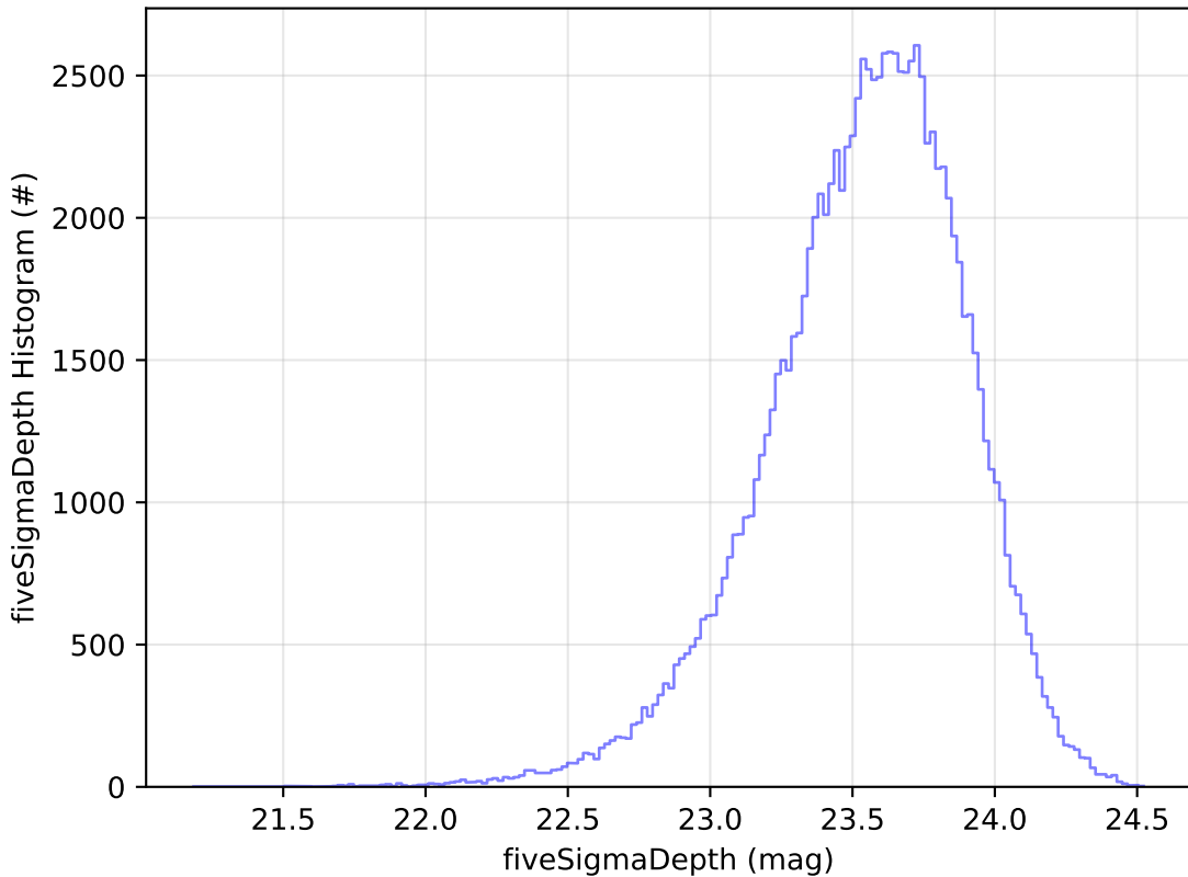
baseline_v3.0_10yrs u: fiveSigmaDepth Histogram
