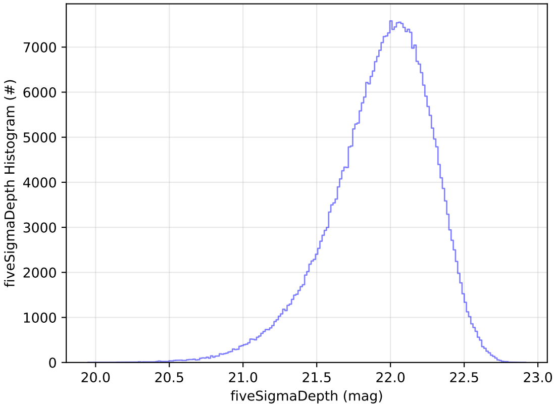
baseline_v3.0_10yrs y: fiveSigmaDepth Histogram
