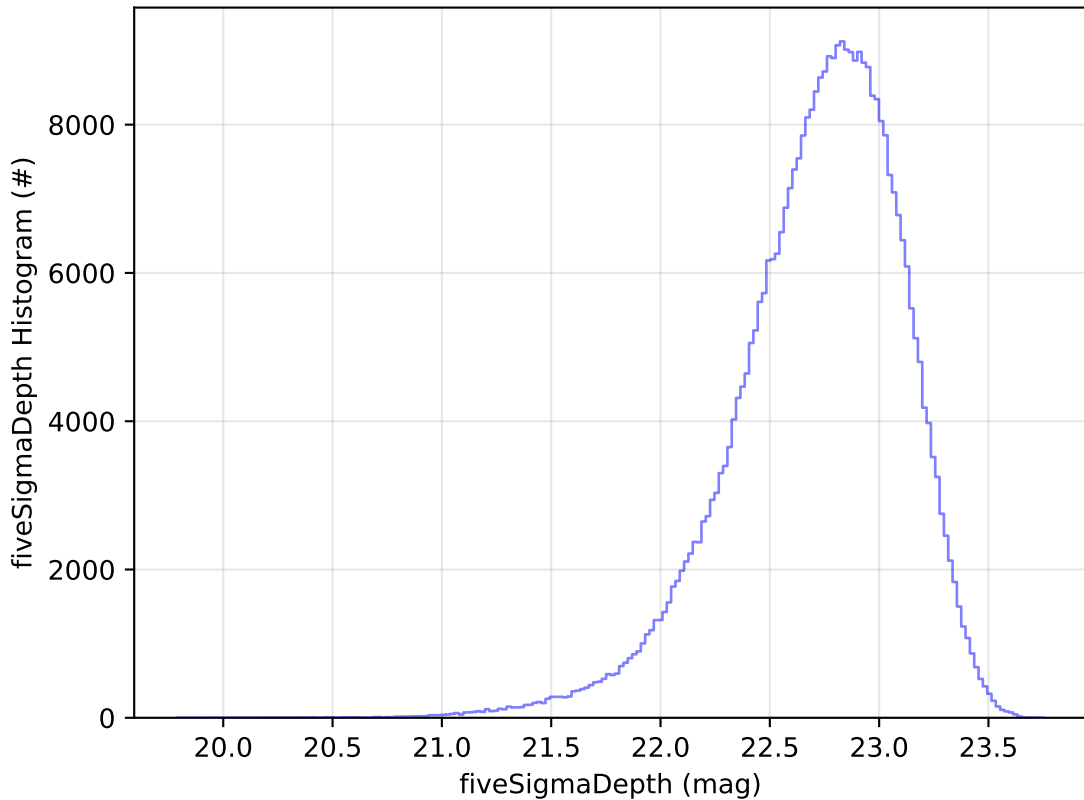
baseline_v3.0_10yrs z: fiveSigmaDepth Histogram
