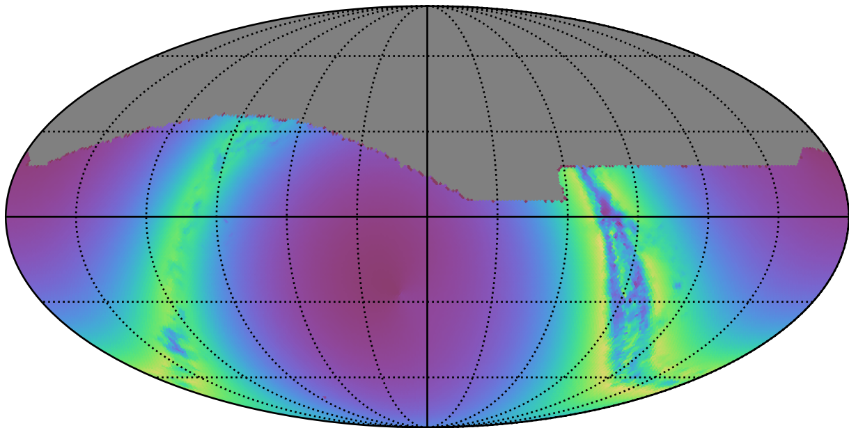
baseline_v3.0_10yrs : young_stars
