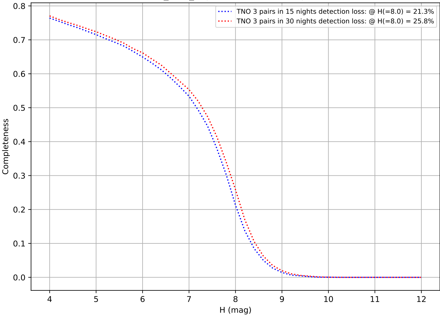
baseline_v3.0_10yrs: DifferentialCompleteness
