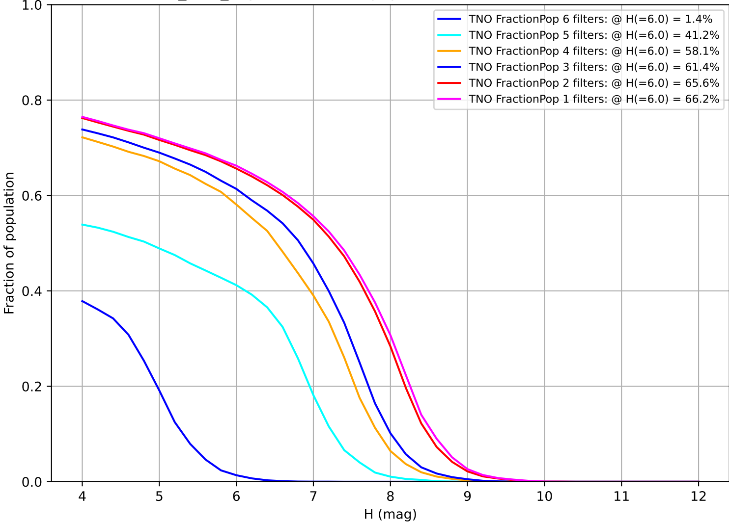
baseline_v3.0_10yrs: Fraction of population with colors in X filters TNO
