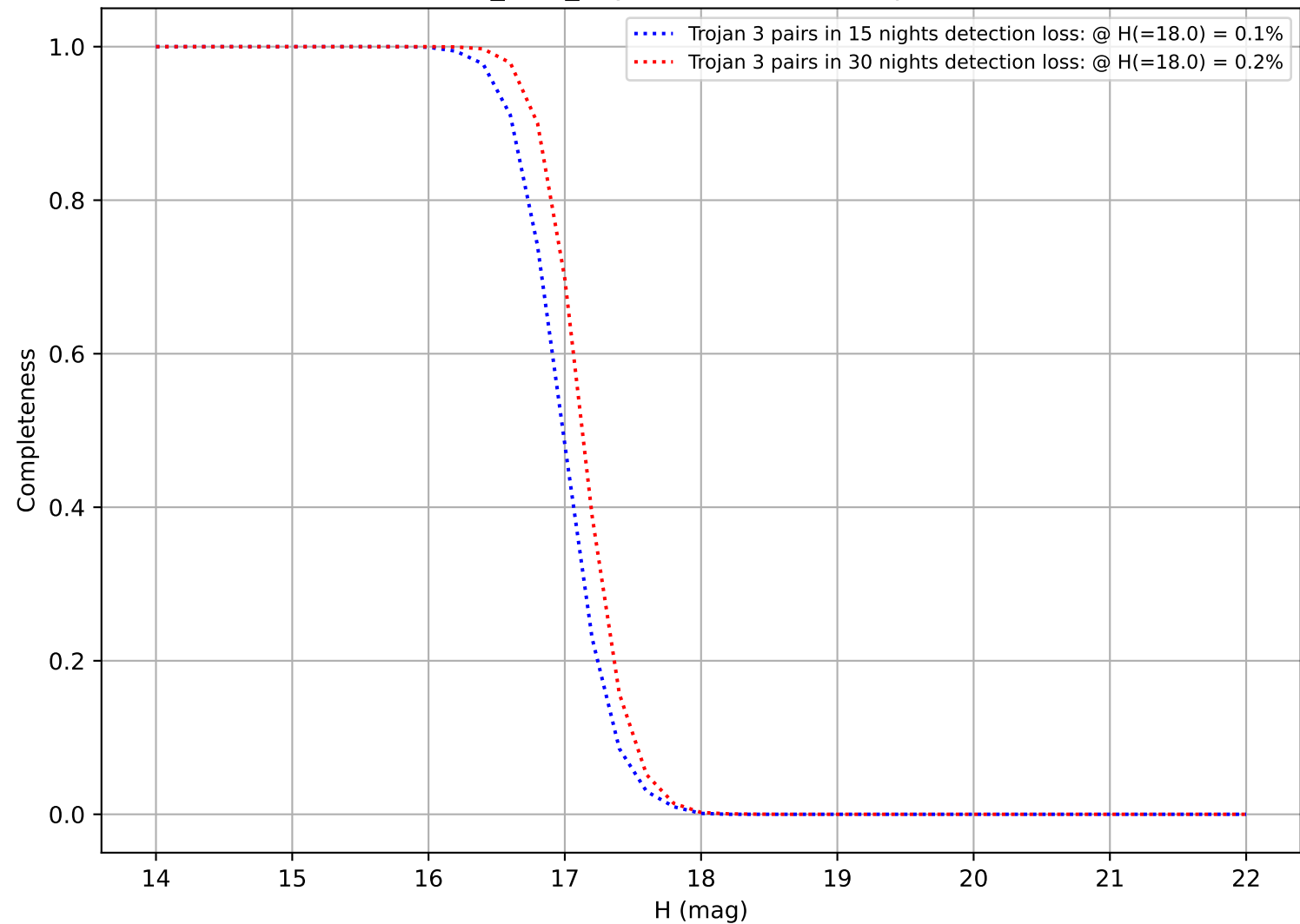
baseline_v3.0_10yrs: DifferentialCompleteness
