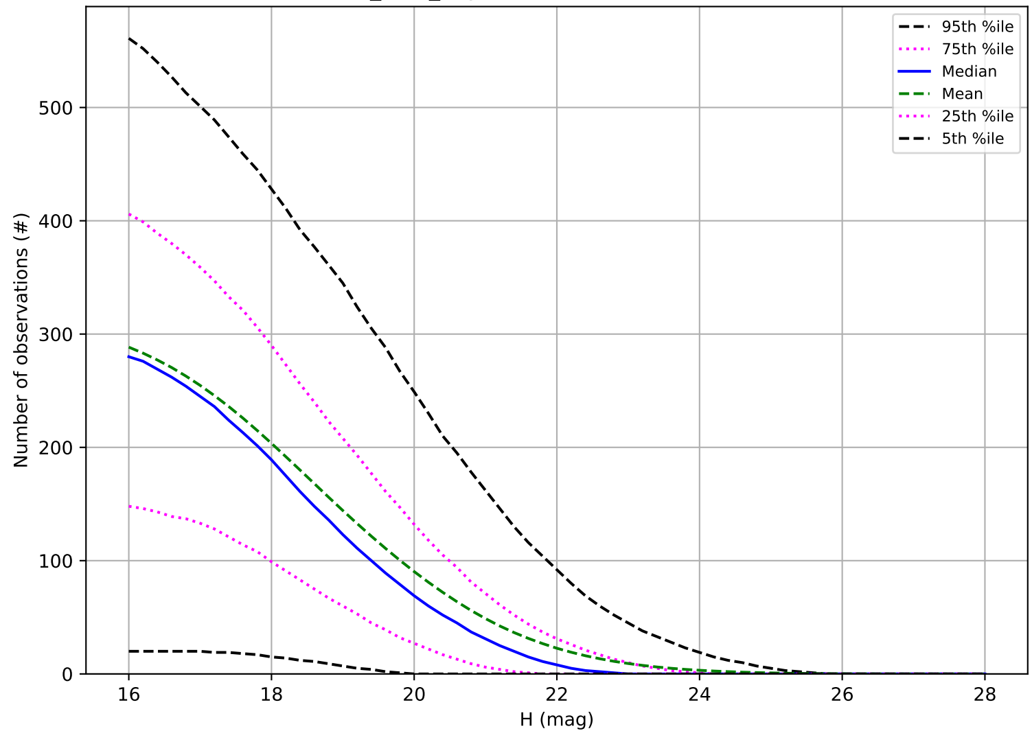
baseline_v3.0_10yrs: Number of observations NEO
