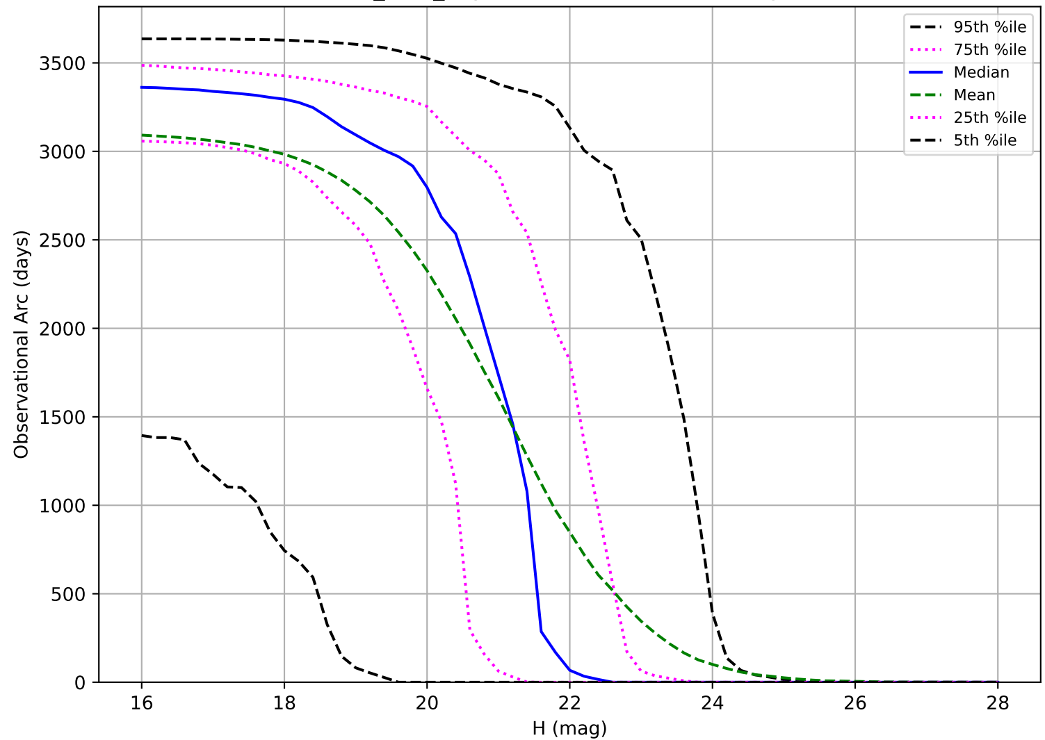
baseline_v3.0_10yrs: Observational Arc Length NEO
