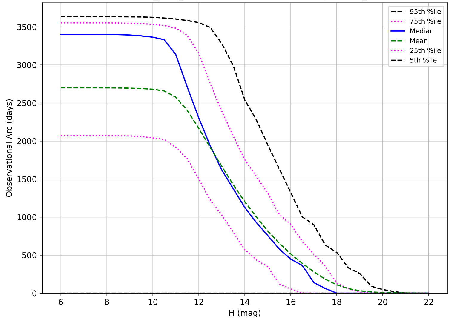
baseline_v3.0_10yrs: Observational Arc Length OCC_r5
