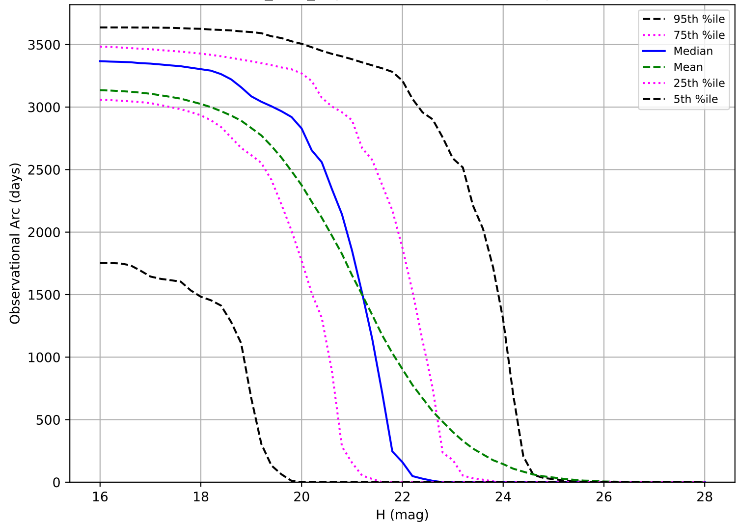
baseline_v3.0_10yrs: Observational Arc Length PHA
