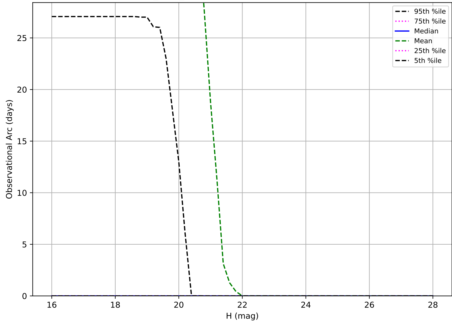
baseline_v3.0_10yrs: Observational Arc Length Vatira
