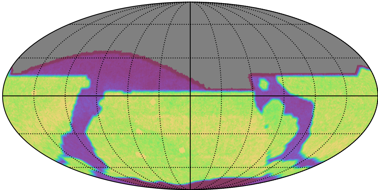
baseline_v3.2_10yrs : Count observationStartMJD
