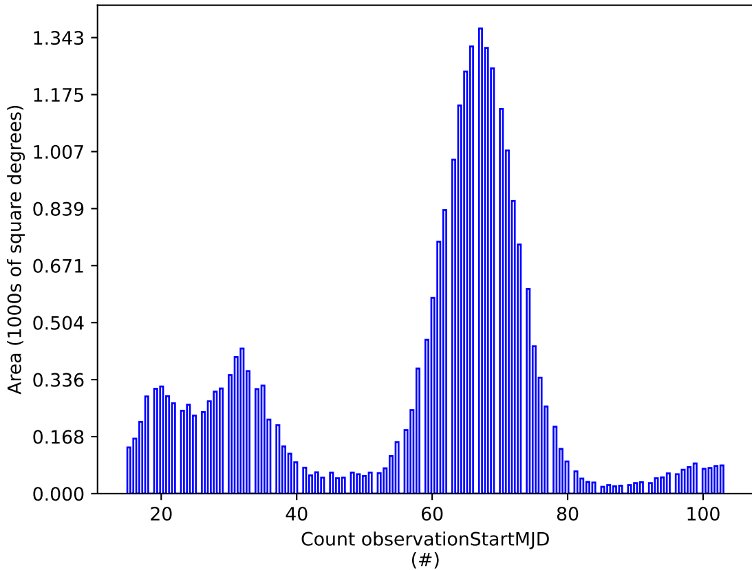
baseline_v3.2_10yrs g: Count observationStartMJD
