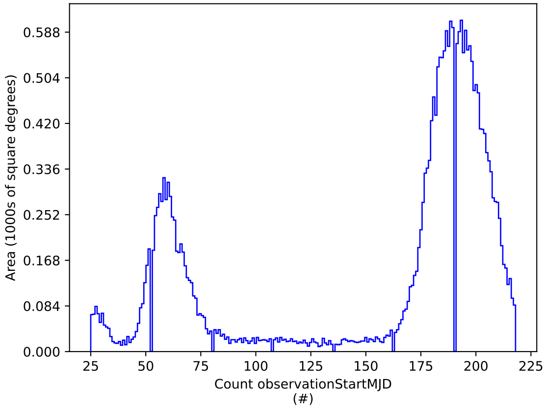
baseline_v3.2_10yrs i: Count observationStartMJD
