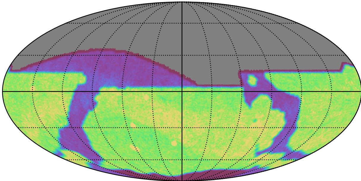
baseline_v3.2_10yrs i: Count observationStartMJD
