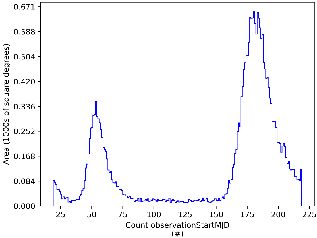
baseline_v3.2_10yrs r: Count observationStartMJD
