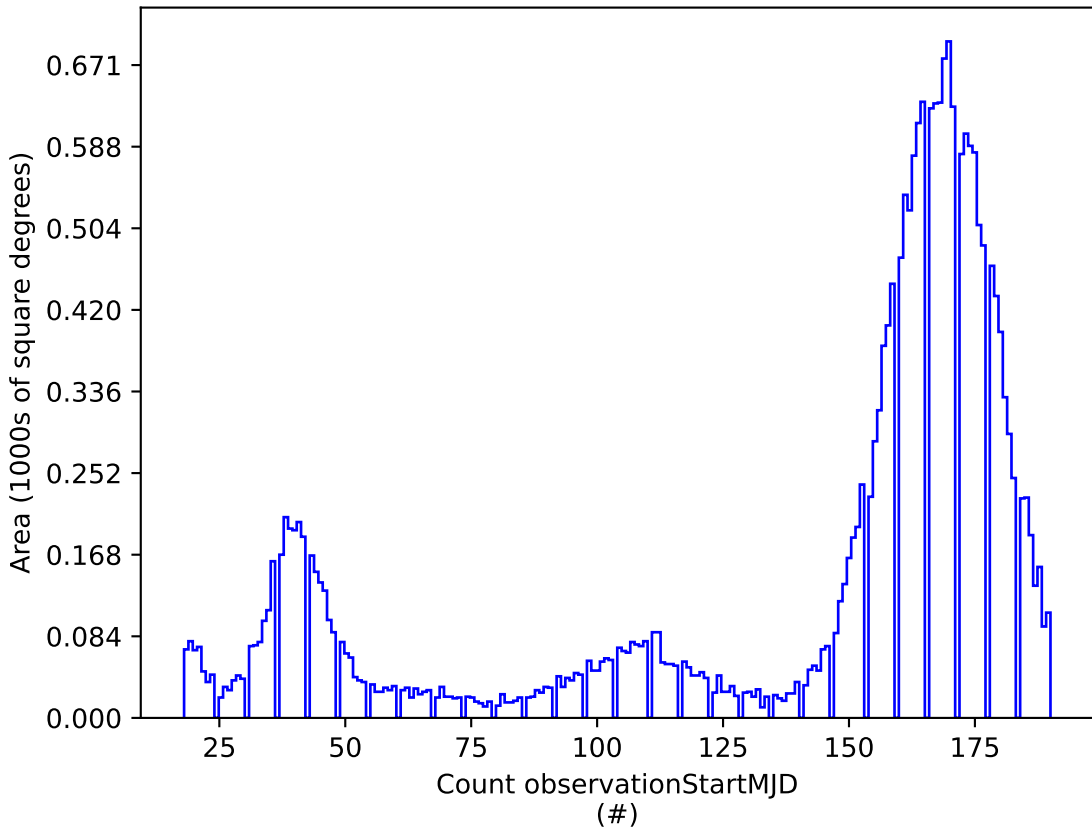
baseline_v3.2_10yrs y: Count observationStartMJD
