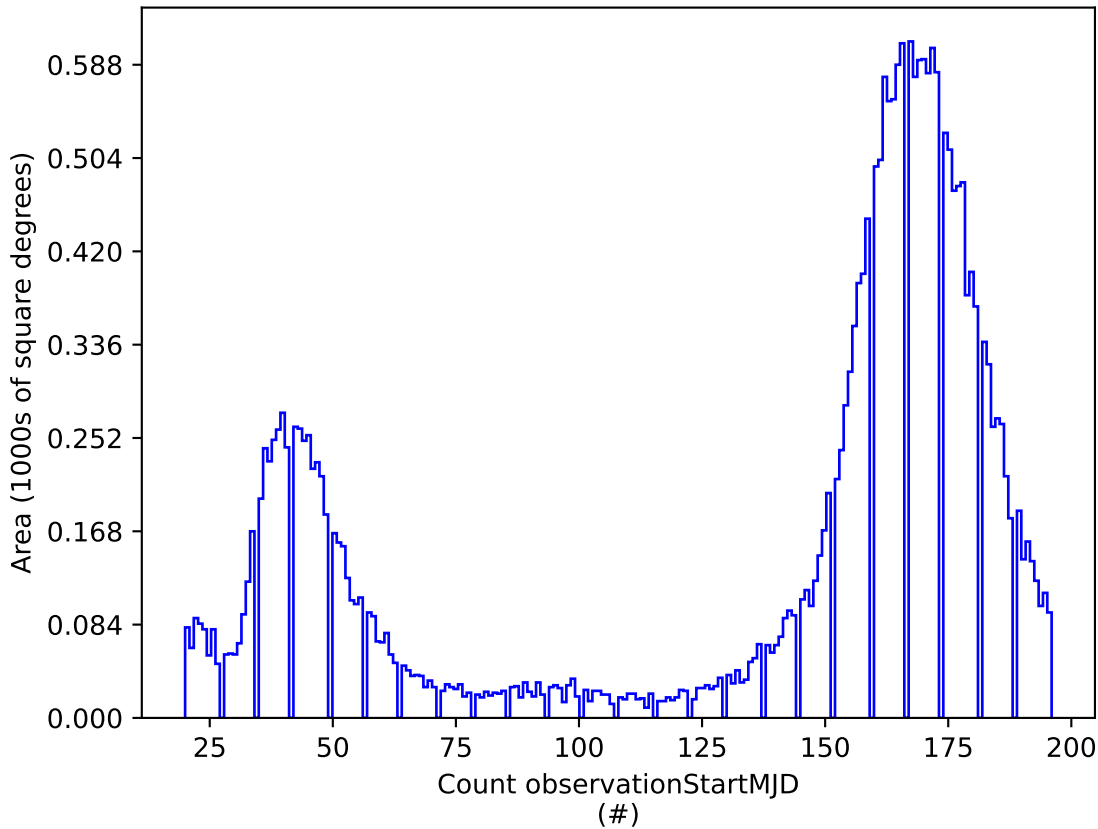
baseline_v3.2_10yrs z: Count observationStartMJD
