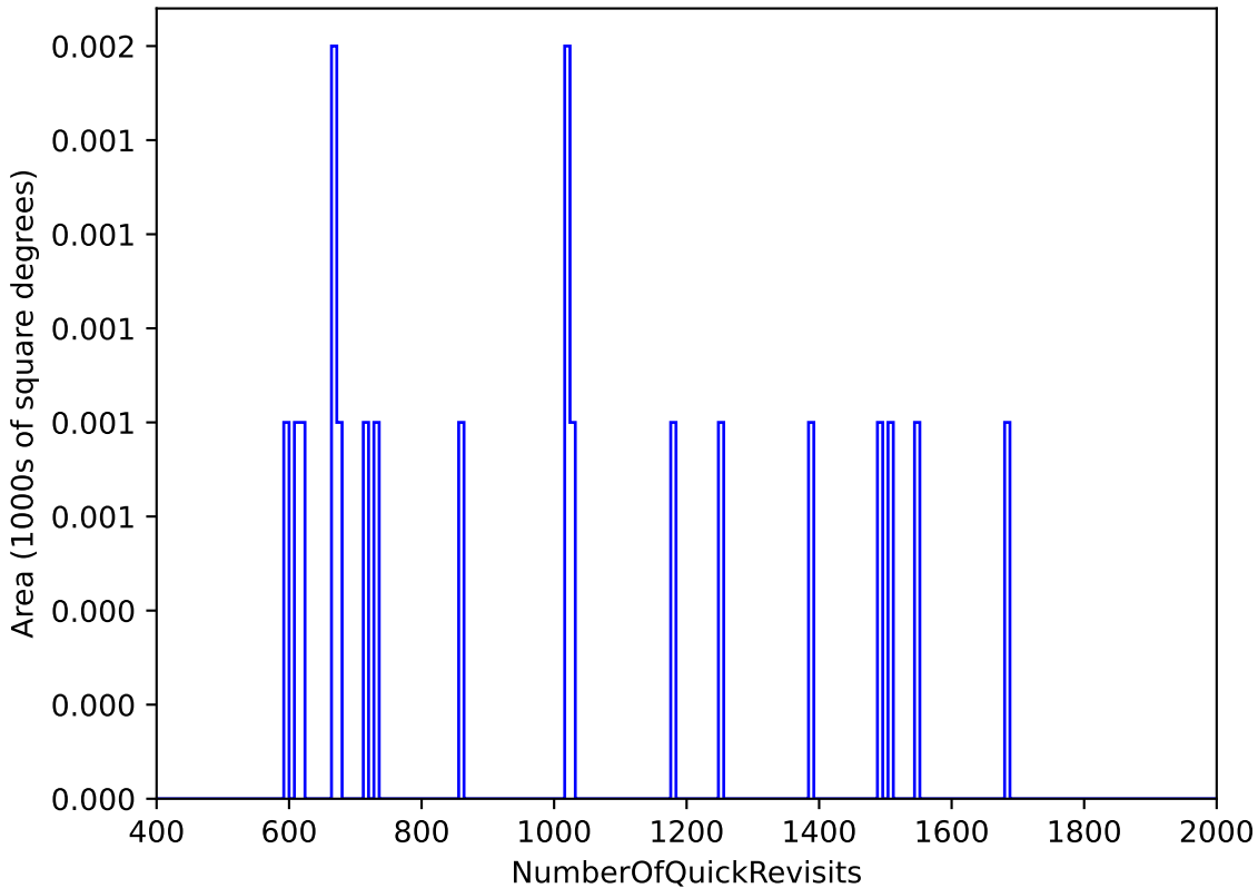
baseline_v3.2_10yrs WFD: NumberOfQuickRevisits
