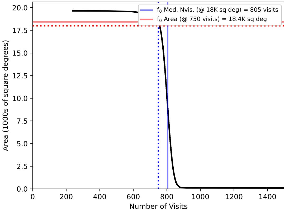
baseline_v3.2_10yrs WFD: f0
